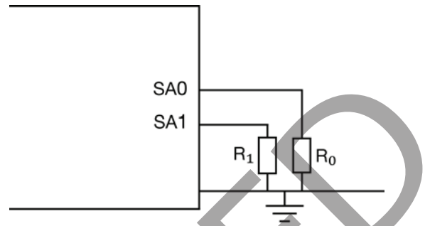
Schematic of connection of address resistors.
