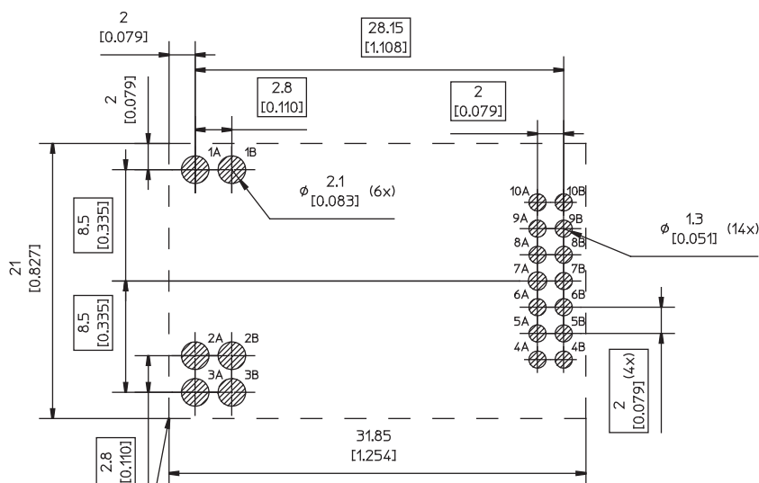
Recommended keep out area for user components
