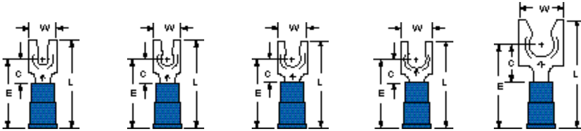
Stud Size MV14-4FL MV14-6FL MV14-8FL MV14-10FL MV14-14FL 4 6 8 10 1/4 Wire Range 16-14 16-14 16-14 16-14 16-14
