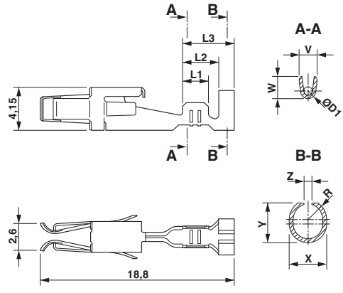
Dimensional drawing
