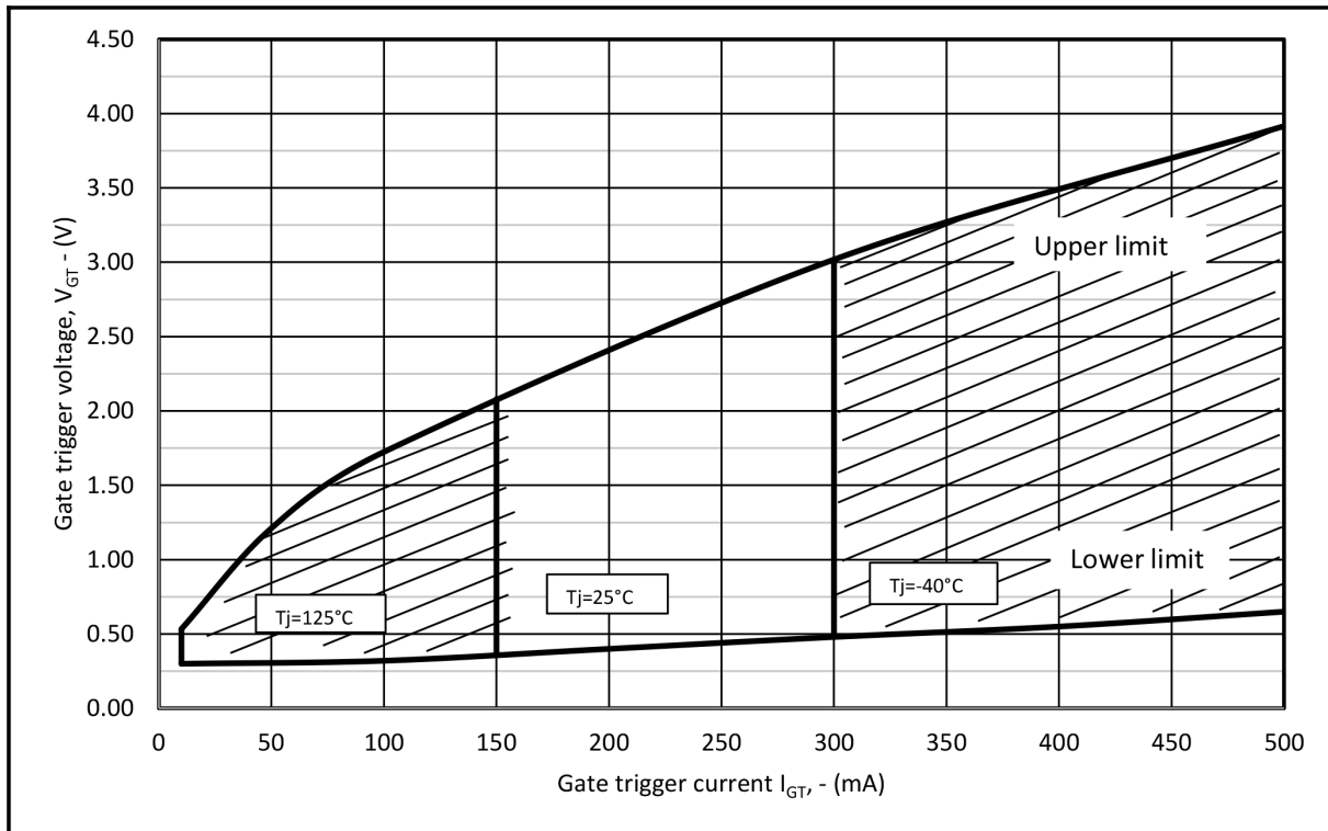
Fig.12 Gate characteristics
