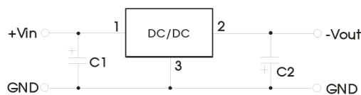
Negative output application circuit
