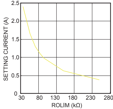
Programmable Output Current Limit (I OLIM vs. R OLIM )
