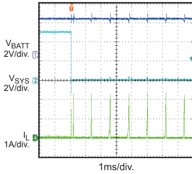
SYS short Entry Boost Mode
