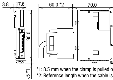
FC5A-EXM1M
