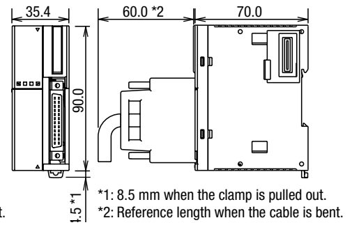
FC5A-EXM1S
