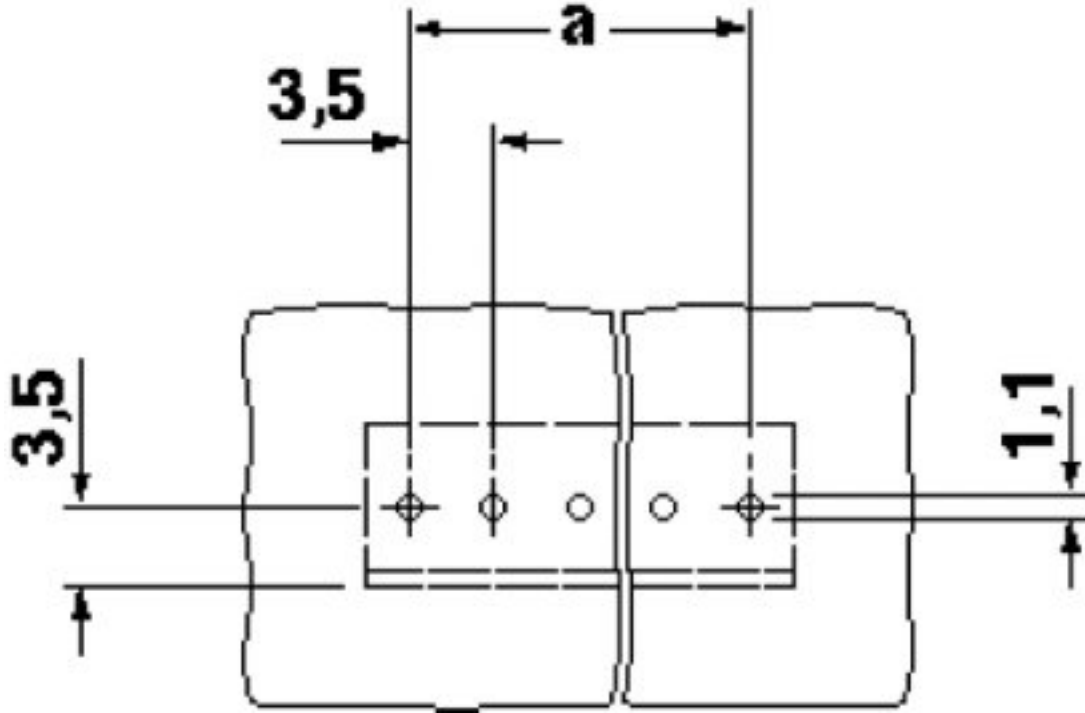
Drilling diagram
