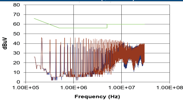
MGJ2D122005MPC (Quasi-Peak)
