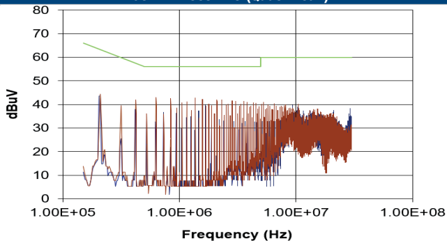
MGJ2D121509MPC (Quasi-Peak)
