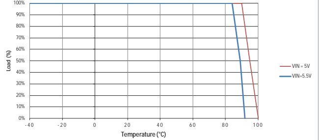
MGJ2D051509MPC
