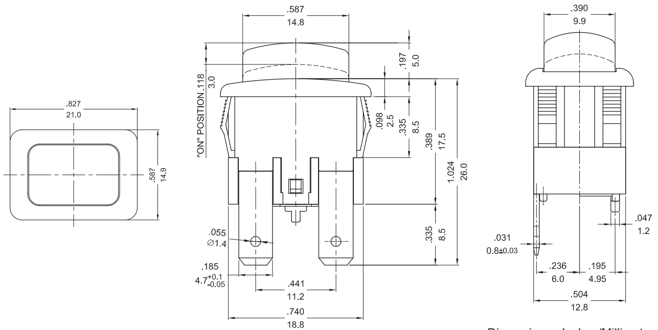
Dimensions : Inches/Millimetres Tolerances \pm 0.012"/0.3\text{mm}
