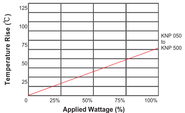
Temperature Rise
