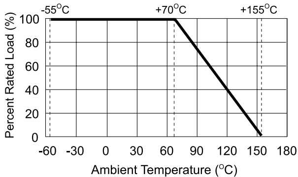
Derating Curve
