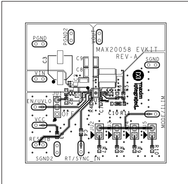
Component Placement Guide—Top
