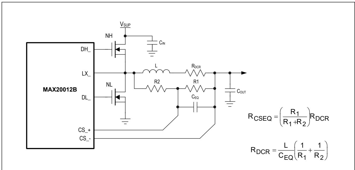
Figure 8. Current-Sense Configurations
