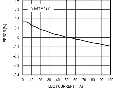
LDO1 LOAD REGULATION
