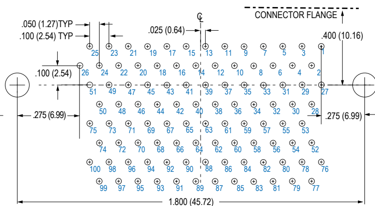
100 SOCKET M83513/15-H
