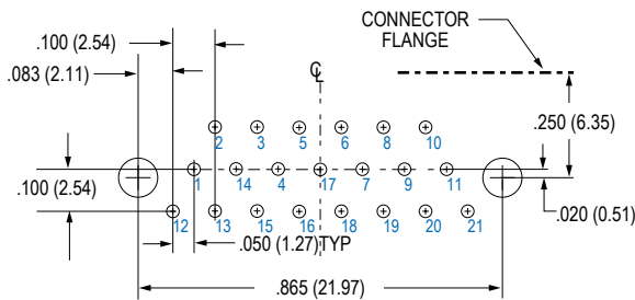
21 PIN M83513/10-C
