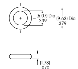
AT401P O-ring for Splashproof Models Natural Rubber
