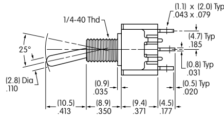
M2011 model does not have terminal 1.
