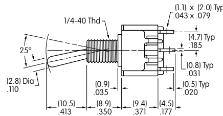
M2021 model does not have terminals 1 & 4.
