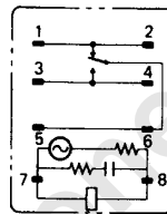
Terminal arrangement/Internal connections (Bottom view)
