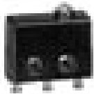
SX Series Subminiature Basic Switch, Single Pole Double Throw (SPDT), 28 Vdc, 7 A, Pin Plunger Actuator, Solder Termination
