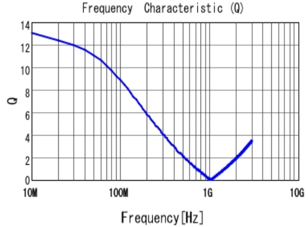
■ LQW18CAR33J00 Q
