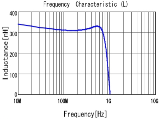
■ LQW18CAR33J00 L
