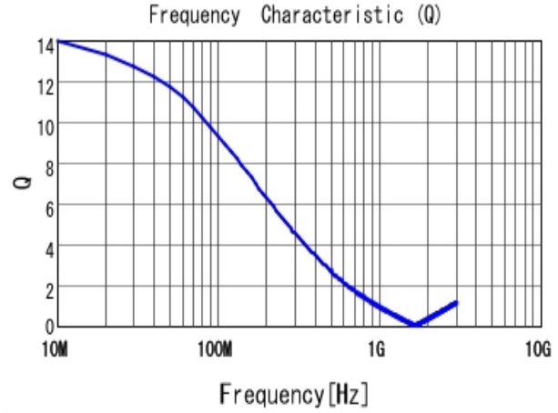
■ LQW18CAR12J00 Q
