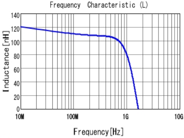
■ LQW18CAR12J00 L
