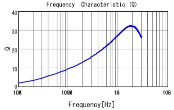
■ LQP03TN9N1H02 Q
