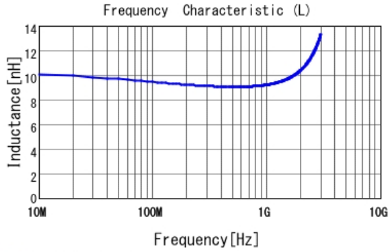
■ LQP03TN9N1H02 L
