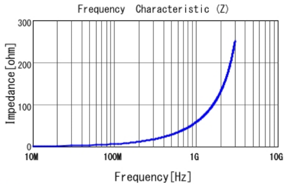
■ LQP03TN9N1H02 |Z|
