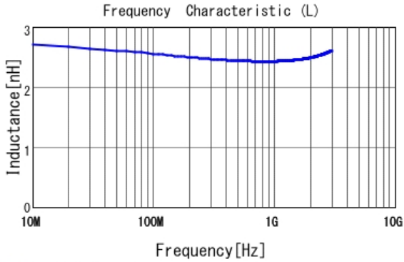
■ LQP03TN2N4B02 L
