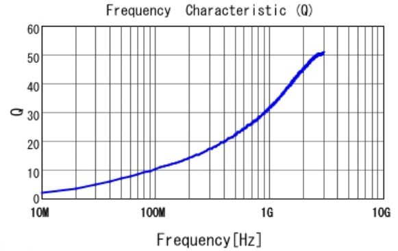
■ LQP03TN2N4B02 Q
