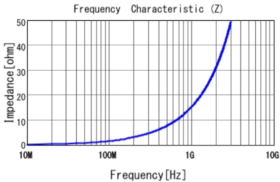
■ LQP03TN2N4B02 |Z|
