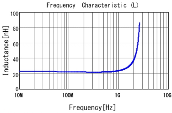
■ LQP03TN22NJ02 L
