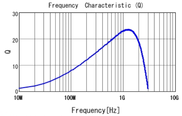
■ LQP03TN22NJ02 Q
