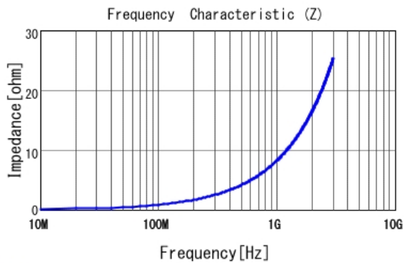
■ LQP03TN1N3B02 |Z|
