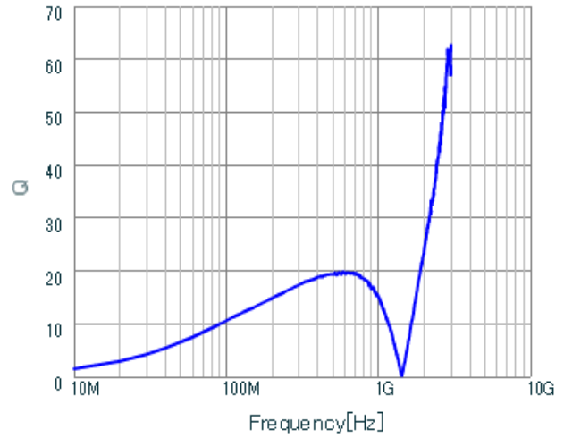
LQP03HQR11J02 Q.
