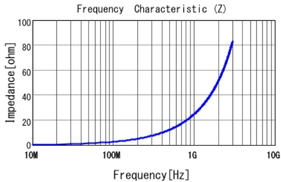
■ LQP03HQ3N9B02 |Z|
