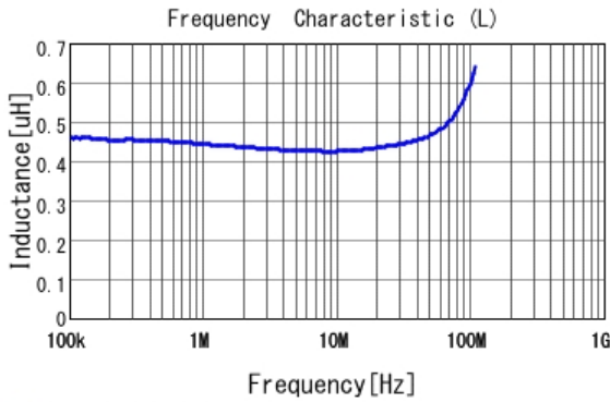
■ LQM2MPNR47NG0 L
