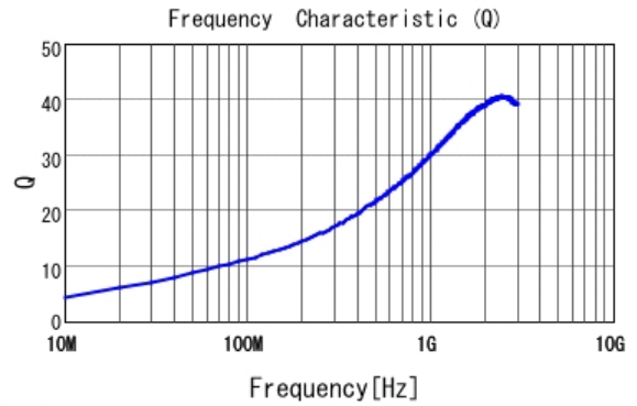
■ LQG15HS4N3S02 Q
