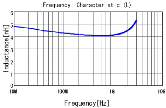
■ LQG15HS4N3S02 L
