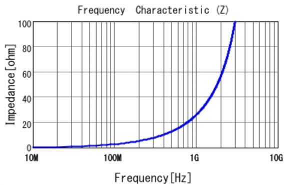
■ LQG15HS4N3S02 |Z|
