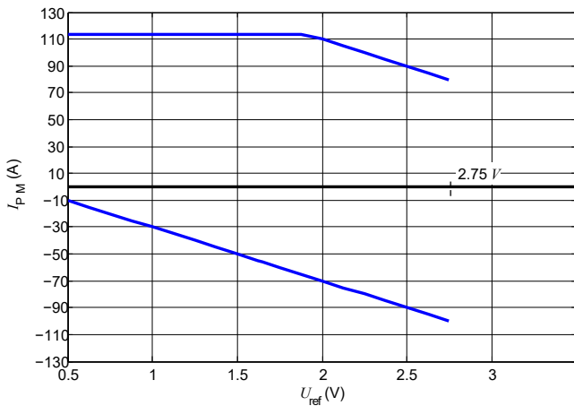
Figure 32: Measuring range versus external U_{ref} LKSR 25 A
