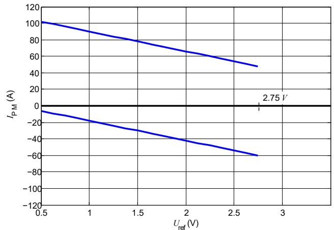
Figure 31: Measuring range versus external U_{ref} LKSR 15 A
