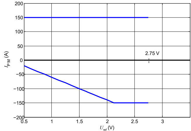
Figure 33: Measuring range versus external U_{ref} LKSR 50 A
