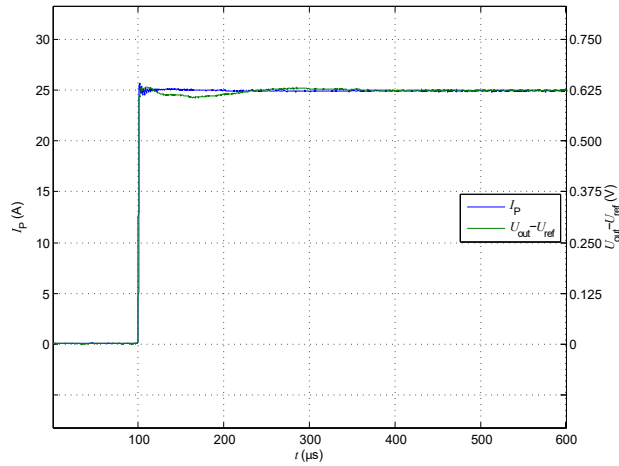
Figure 13: Delay time
