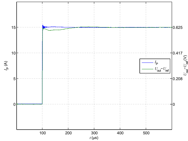
Figure 8: Delay time
