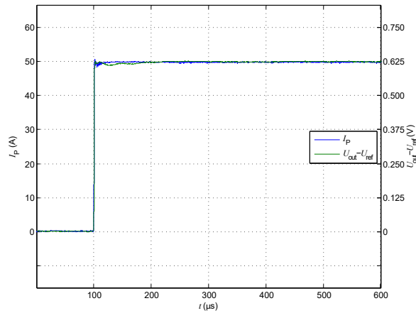
Figure 18: Delay time
