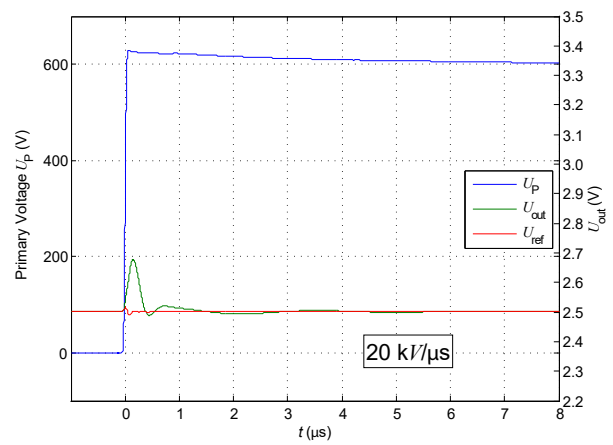
Figure 10: dv/dt
