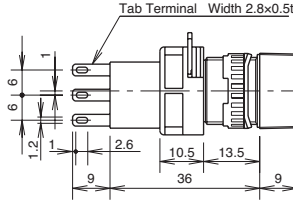
Solder/Tab Terminal
