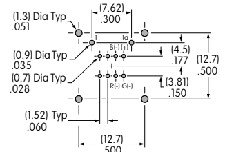
Terminal Detail
