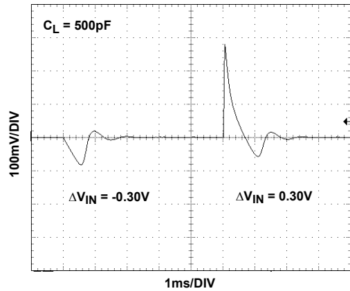
FIGURE 21. LINE TRANSIENT RESPONSE WITH CAPACITIVE LOAD
