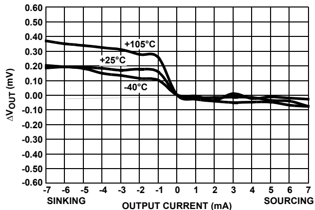
FIGURE 107. LOAD REGULATION
