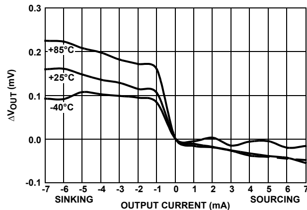
FIGURE 37. LOAD REGULATION
