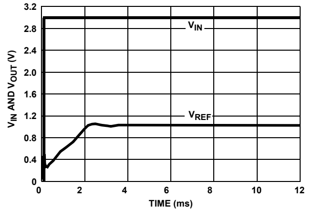
FIGURE 13. TURN-ON TIME (+25°C)
