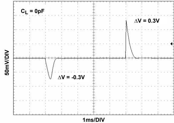
FIGURE 63. LINE TRANSIENT RESPONSE
