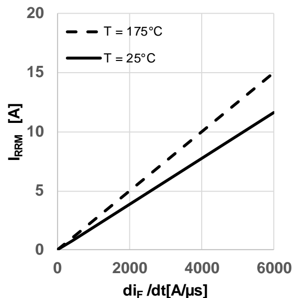
Figure 20 Typical reverse recovery current as a function of diode current slope (I_{rrm} = f(di_i/dt), V_{DD} = 800V, V_{GS} = 0V/18V, I_D = 8.5A, \text{ ind. load, test circuit in Fig.E,} body diode at V_{GS} = 0V)
