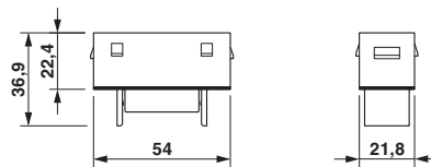
Dimensional drawing
