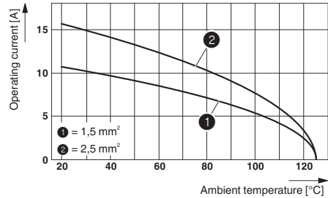
Derating diagram (6 modules in HC-B 24 housing)
