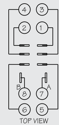
TERMINAL LOCATION
