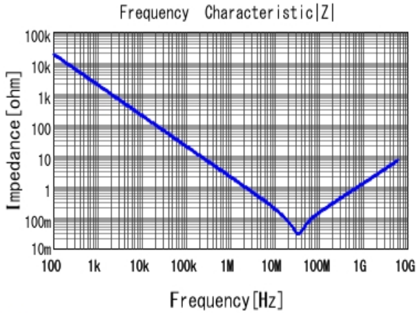
■ GRT033R60J104KE01 |Z| DCOV, 25degC
