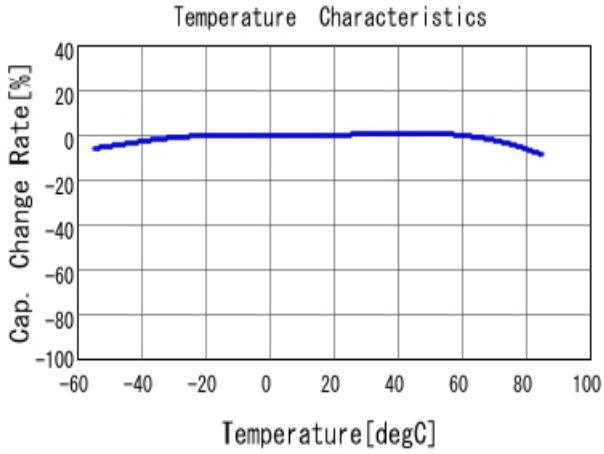
■ GRT033R60J104KE01 C-Temp. capchange, DC0.0V, AC0.5V rm
