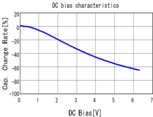
■ GRT033R60J104KE01 C-DC bias capchange, 25.0degC, AC0.
