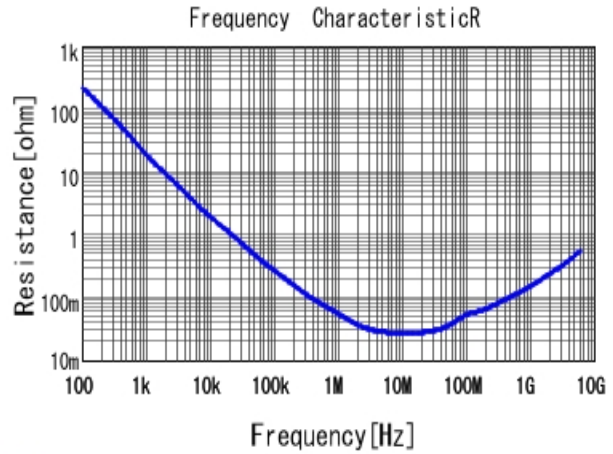
■ GRT033R60J104KE01 R DCOV, 25degC
