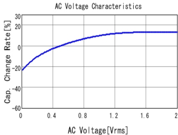
■ GRT033R60J104KE01 C-AC Voltage capchange, DCOV, 25.0d
