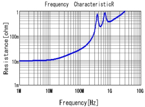
■ GRM32A7U2J222JW31 R DCOV, 25degC
