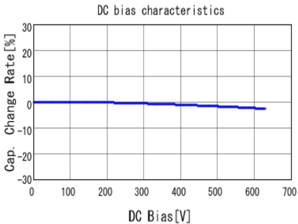
■ GRM32A7U2J222JW31 C-DC bias capchange, 25.0degC, AC1V
