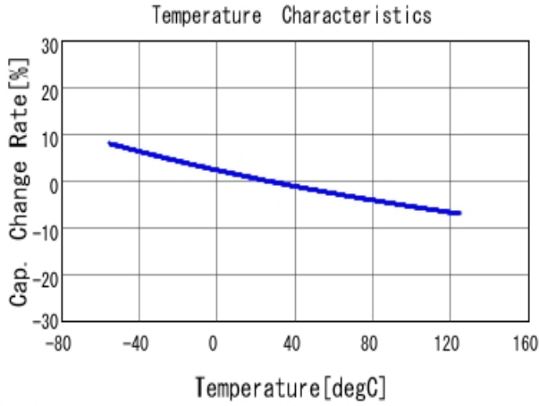
■ GRM32A7U2J222JW31 C-Temp. capchange, DCOV, AC1Vrms
