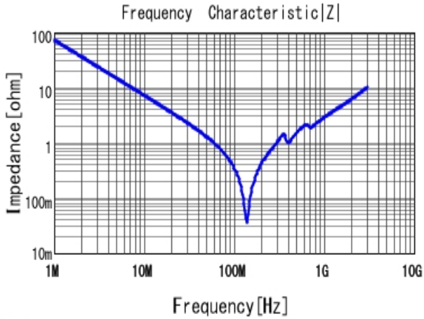
■ GRM32A7U2J222JW31 |Z| DCOV, 25degC
