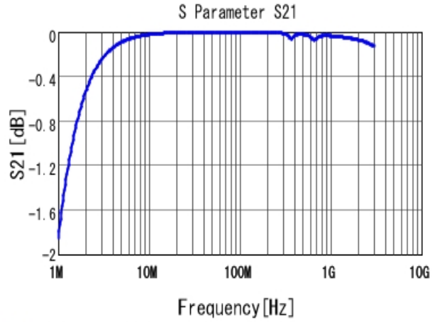
■ GRM32A7U2J222JW31 S21 DCOV, 25degC
