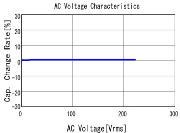
■ GRM32A7U2J222JW31 C-AC Voltage capchange, DCOV, 25.0d
