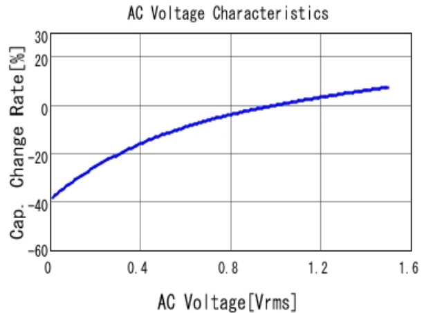
■ GRM31CR71E106KA12 C-AC Voltage capchange, DCOV, 25.0d
