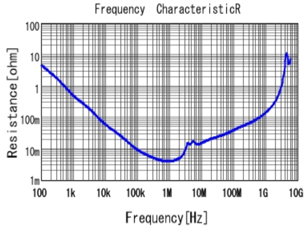
■ GRM31CR71E106KA12 R DCOV, 25degC
