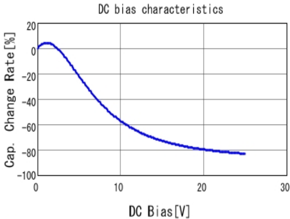
■ GRM31CR71E106KA12 C-DC bias capchange, 25.0degC, AC1.
