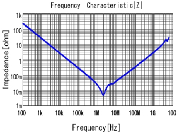
■ GRM31CR71E106KA12 |Z| DCOV, 25degC
