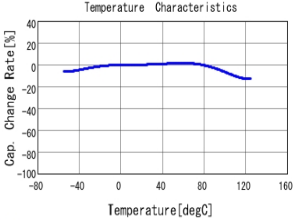
■ GRM31CR71E106KA12 C-Temp. capchange, DCO. 0V, AC1.0V r m
