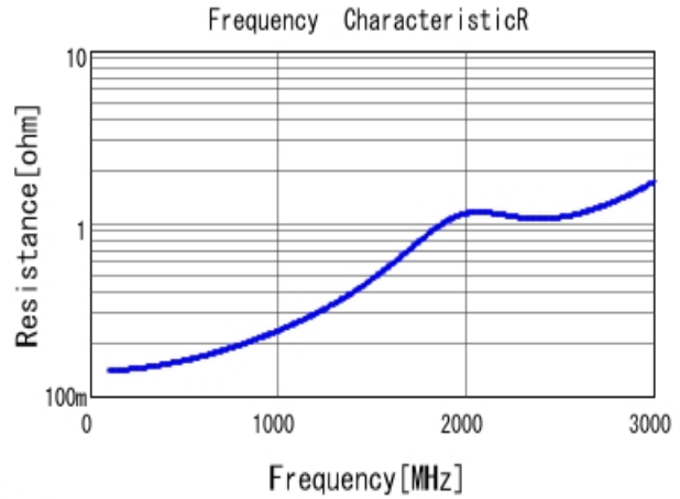
■ GRM31A7U2J101JW31 R DCOV, 25degC
