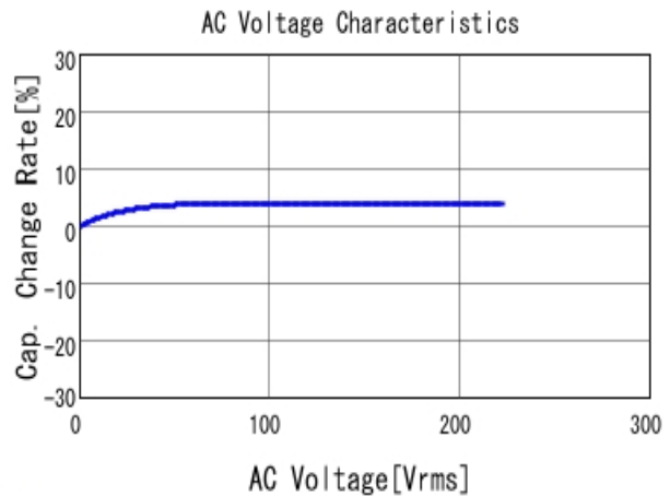
■ GRM31A7U2J101JW31 C-AC Voltage capchange, DCOV, 25.0d
