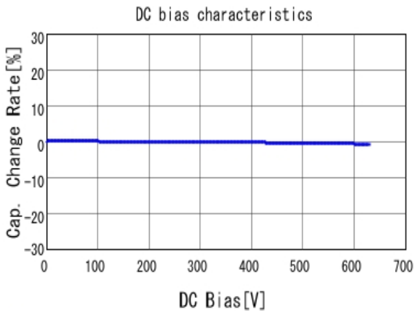
■ GRM31A7U2J101JW31 C-DC bias capchange, 25.0degC, AC1V
