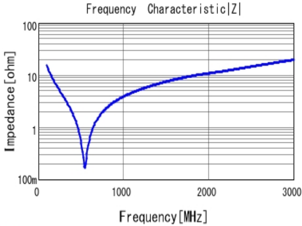
■ GRM31A7U2J101JW31 |Z| DCOV, 25degC
