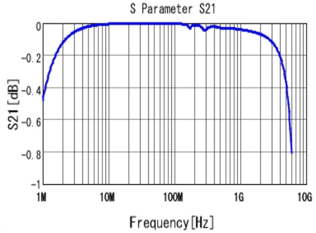
■ GRM3195C2A472JA01 S21 DCOV, 25degC
