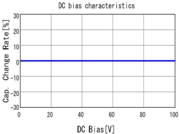
■ GRM3195C2A472JA01 C-DC bias capchange, 25.0degC, AC1V
