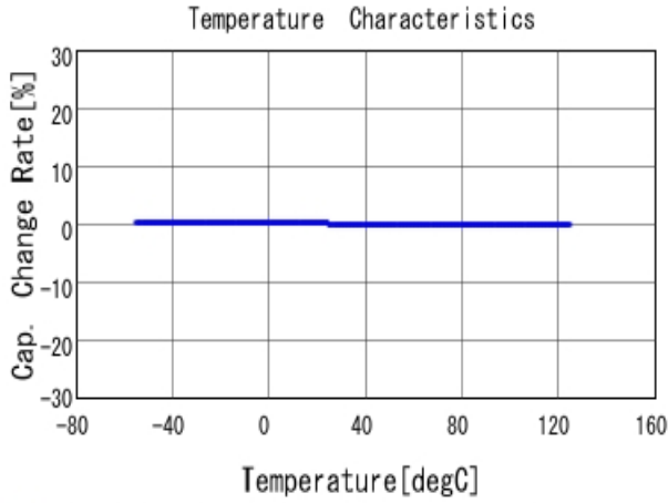
■ GRM3195C2A472JA01 C-Temp. capchange, DCOV, AC1Vrms
