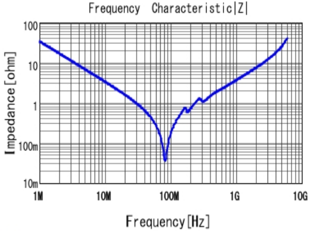
■ GRM3195C2A472JA01 |Z| DCOV, 25degC
