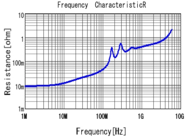
■ GRM3195C2A472JA01 R DCOV, 25degC
