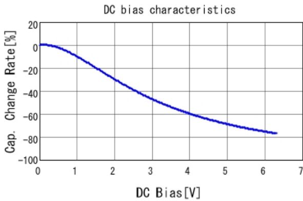
GRM188R60J106ME47 C-DC bias capchange, 25.0degC, A
