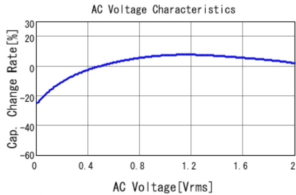
GRM188R60J106ME47 C-AC Voltage capchange, DCOV, 25
