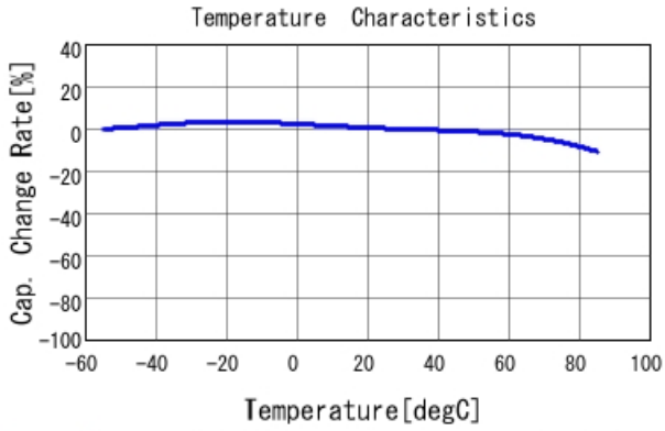
GRM188R60J106ME47 C-Temp. capchange, DC0.0V, AC0.5
