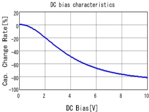
■ GRM188D71A106MA73 C-DC bias capchange, 25.0degC, AC1V
