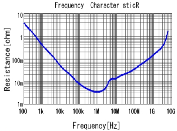
■ GRM188D71A106MA73 R DCOV, 25degC
