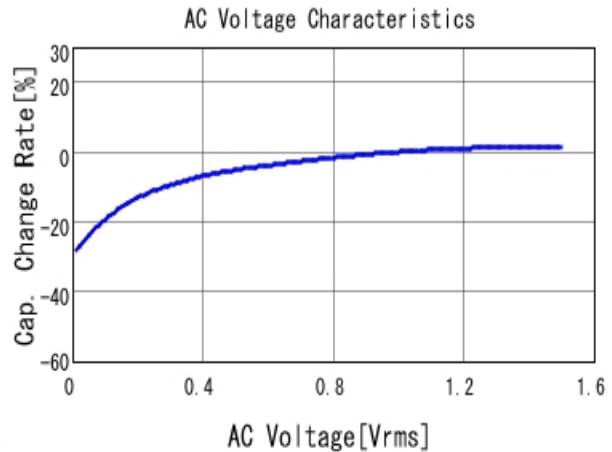
■ GRM188D71A106MA73 C-AC Voltage capchange, DCOV, 25.0d
