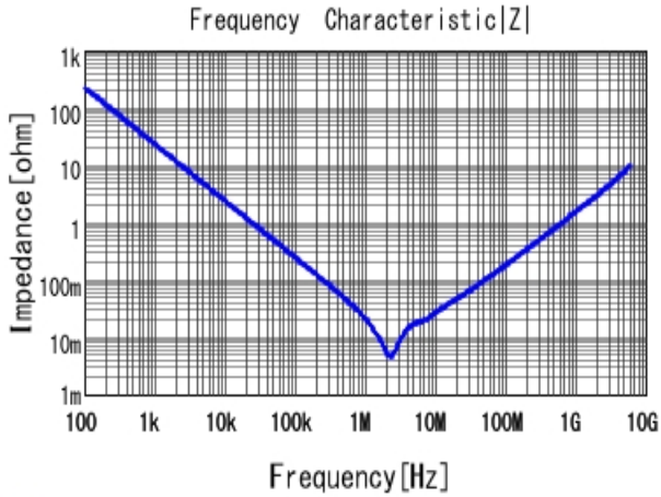
■ GRM188D71A106MA73 |Z| DCOV, 25degC
