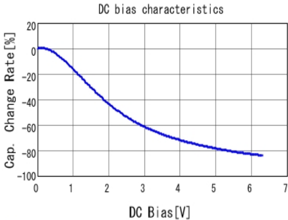
■ GRM033R60J225ME47 C-DC bias capchange, 25.0degC, AC0.
