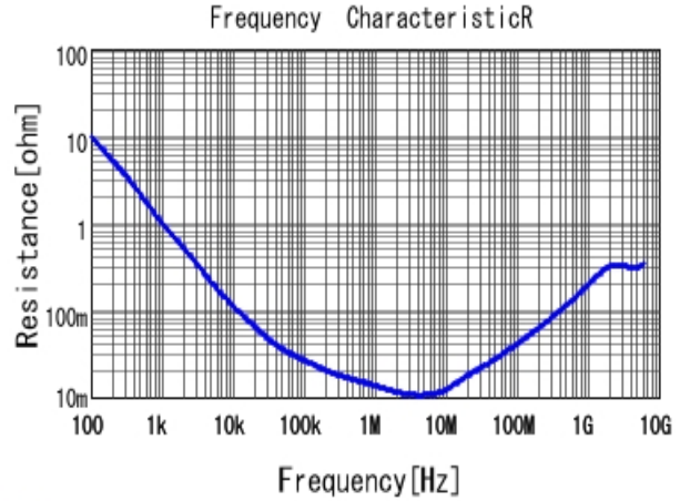
■ GRM033R60J225ME47 R DCOV, 25degC
