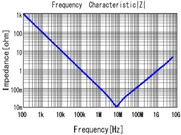
■ GRM033R60J225ME47 |Z| DCOV, 25degC
