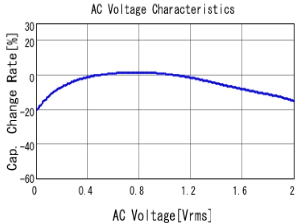
■ GRM033R60J225ME47 C-AC Voltage capchange, DCOV, 25.0d
