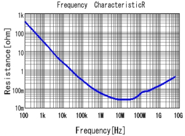
■ GRM033C81A473KE05 R DCOV, 25degC
