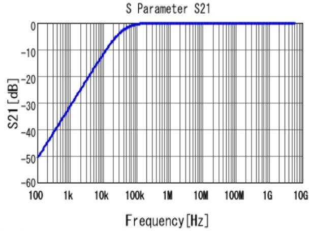
■ GRM033C81A473KE05 S21 DC0V, 25degC
