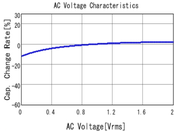
■ GRM033C81A473KE05 C-AC Voltage capchange, DCOV, 25.0d
