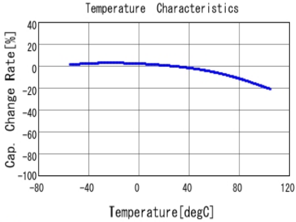
■ GRM033C81A473KE05 C-Temp. capchange, DC0.0V, AC1.0V rm
