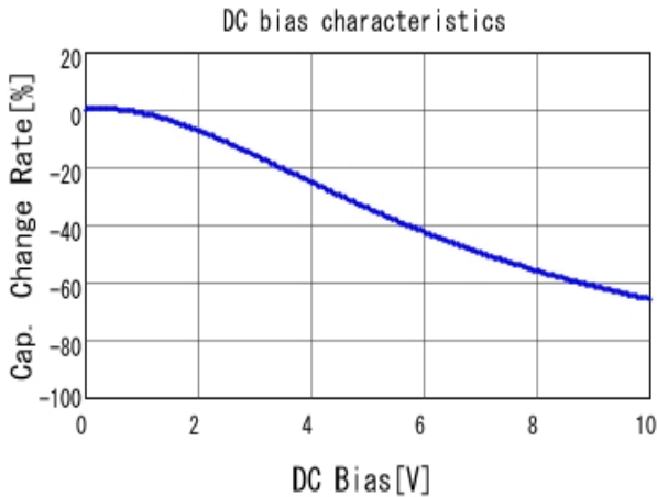
■ GRM033C81A473KE05 C-DC bias capchange, 25.0degC, AC1.
