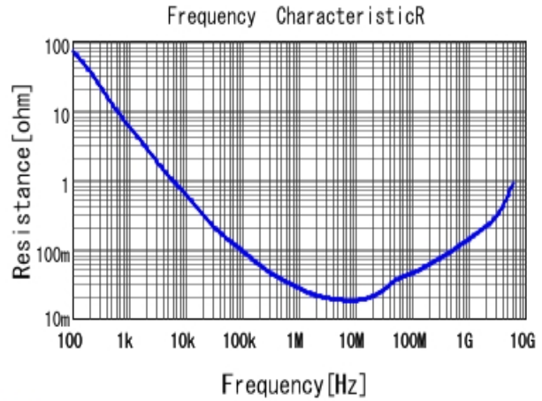
■ GRM033C80J224KE90 R DCOV, 25degC
