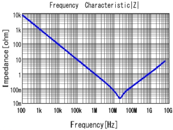
■ GRM033C80J224KE90 |Z| DCOV, 25degC
