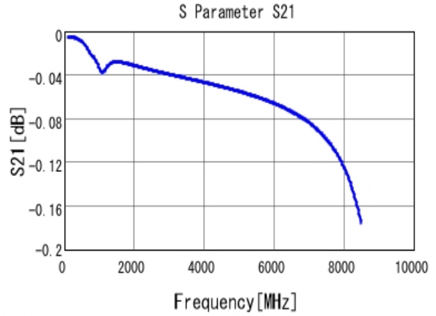
■ GRM0335C1E821GA01 S21 DCOV, 25degC
