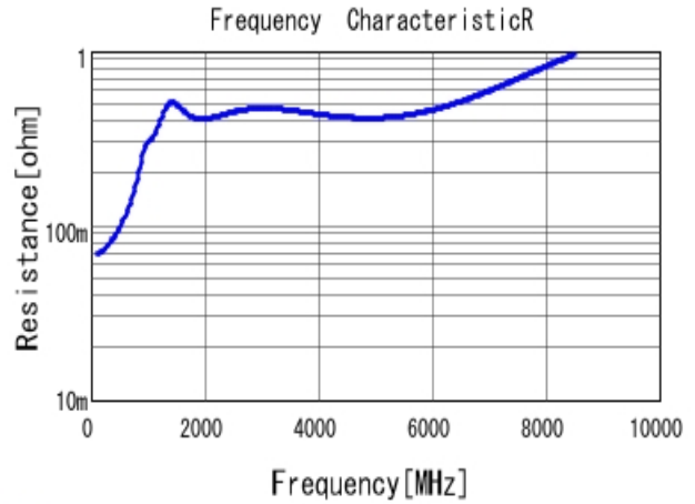
■ GRM0335C1E561JA01 R DCOV, 25degC
